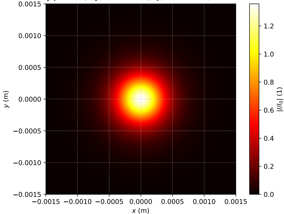
Intensity profile I(x, y, z = 1.513m)/I_0 , \text{Pin}=0.8\text{Pcr} , artificial time
